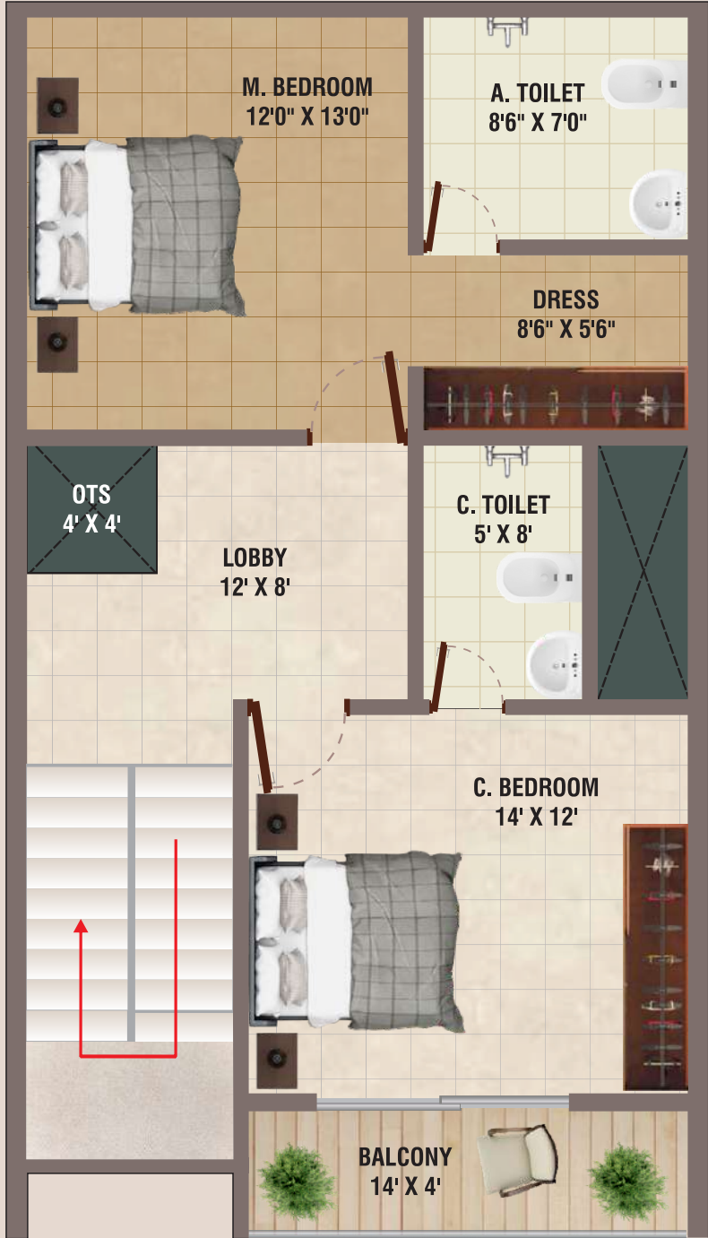
FIRST FLOOR
