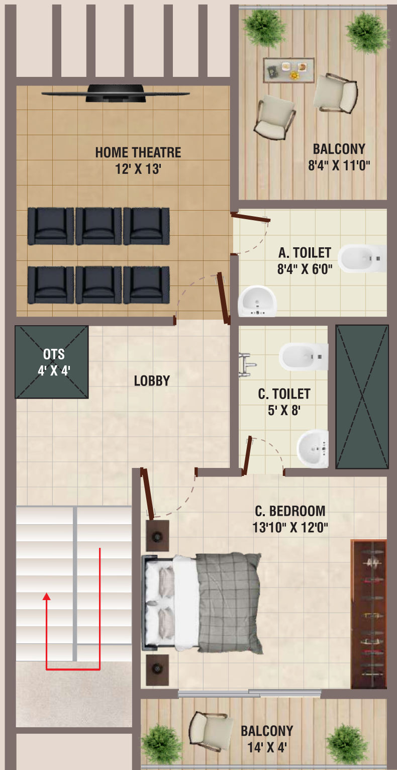
SECOND FLOOR
